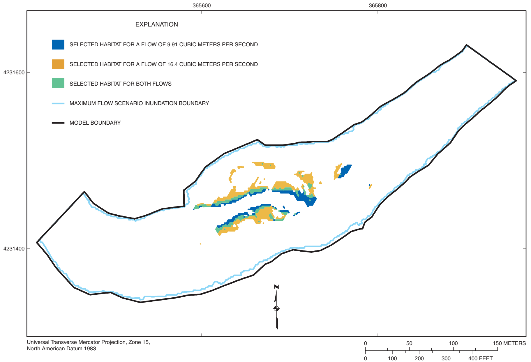
Figure 4-52. Selected habitat area distribution for habitat category 14 (flathead catfish) at flows of 9.91 and 16.4 cubic meters per second at Marais des Cygnes River site MDC2.
